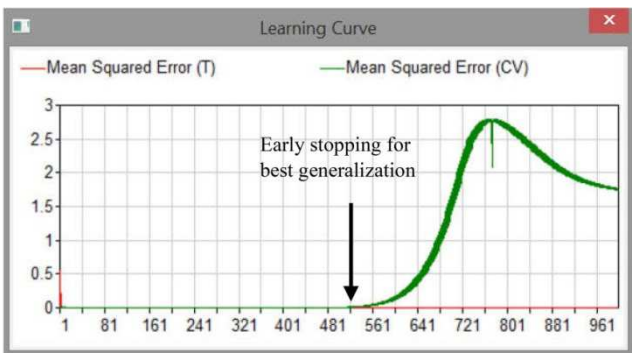
Figure 2. Cross validation (early stopping) during learning curve.
